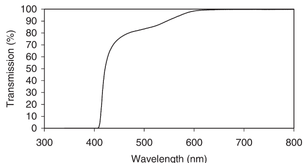
Figure 3. Linear transmission spectrum of 0.94 M thiophene 5 in THF
