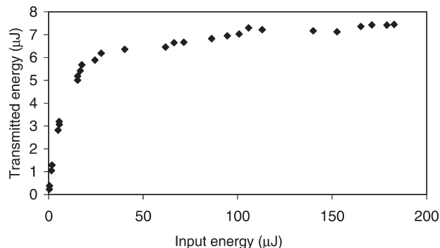
Figure 2. Optical limiting at 532 nm of 0.5 M thiophene 5 in THF
