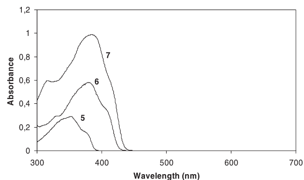
Figure 1. Absorption spectra for thiophenes 5–7 in THF
