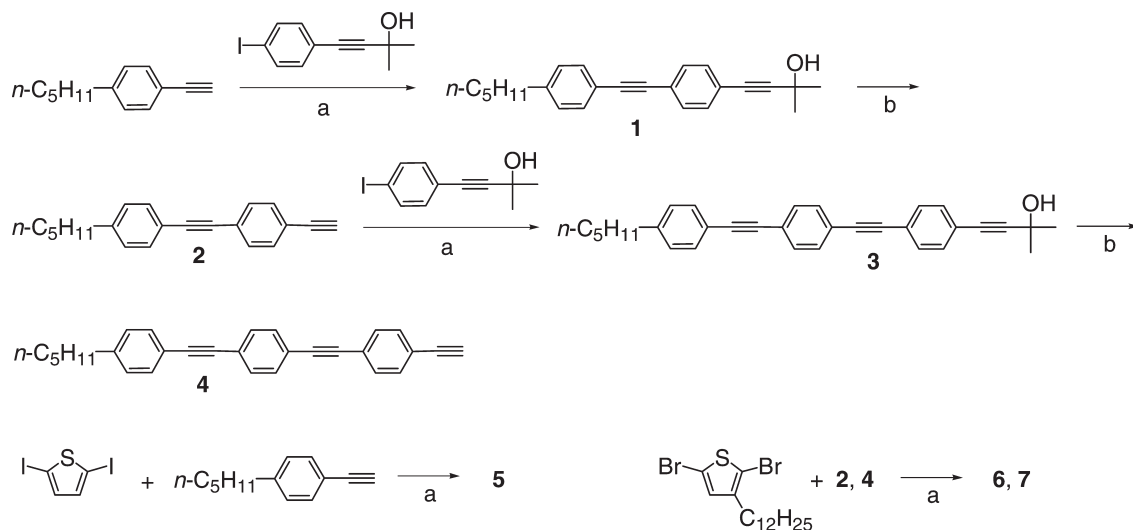
Scheme 2. Reagents and solvents: (a) \text{PdCl}_2(\text{PPh}_3)_2 , CuI, \text{PPh}_3 , pyridine, triethylamine; (b) NaH, \text{C}_6\text{H}_6
